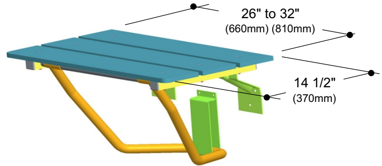
Configuration #62 Adult Folding Shower Seat Shown
